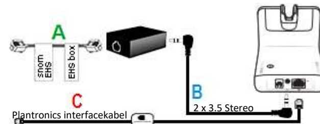
snom EHS adapter
